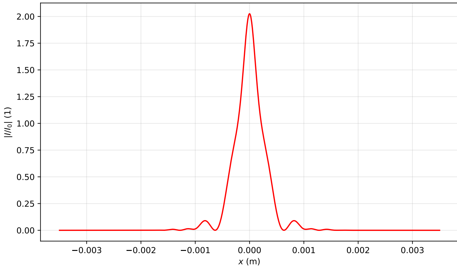
Intensity profile I(x, y = 0, z = 1.194)/I_0 , P_{in}=3.5P_{cr} , artificial time
